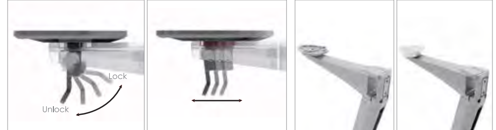
E-Stilts table arm come with locking mechanism, to attach to table top without bolts and nuts with approximately 10 mm of free movement. This table arm also can be applied in Trendx Pro System.
